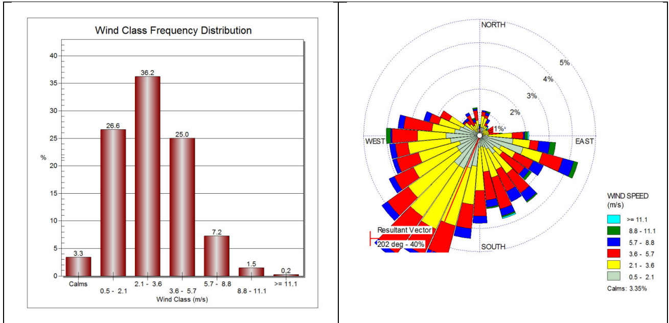
Figure No: 6.2 Wind Rose Diagram & Wind Class Distribution from 6 – 14 Hours
