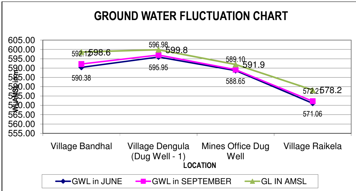
Figure No 6.10 : Seasonal Fluctuation of Ground Water Level
