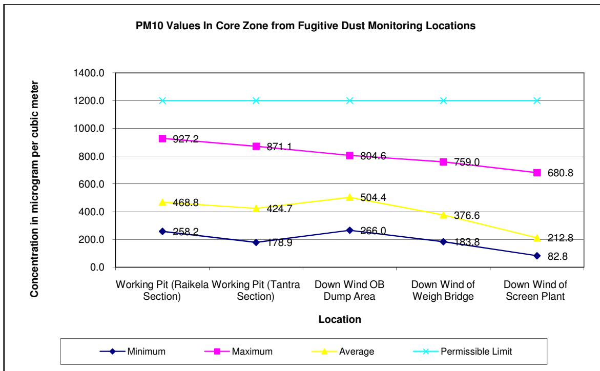
Figure No: 6.9 Graphical Representations of PM10 Values
