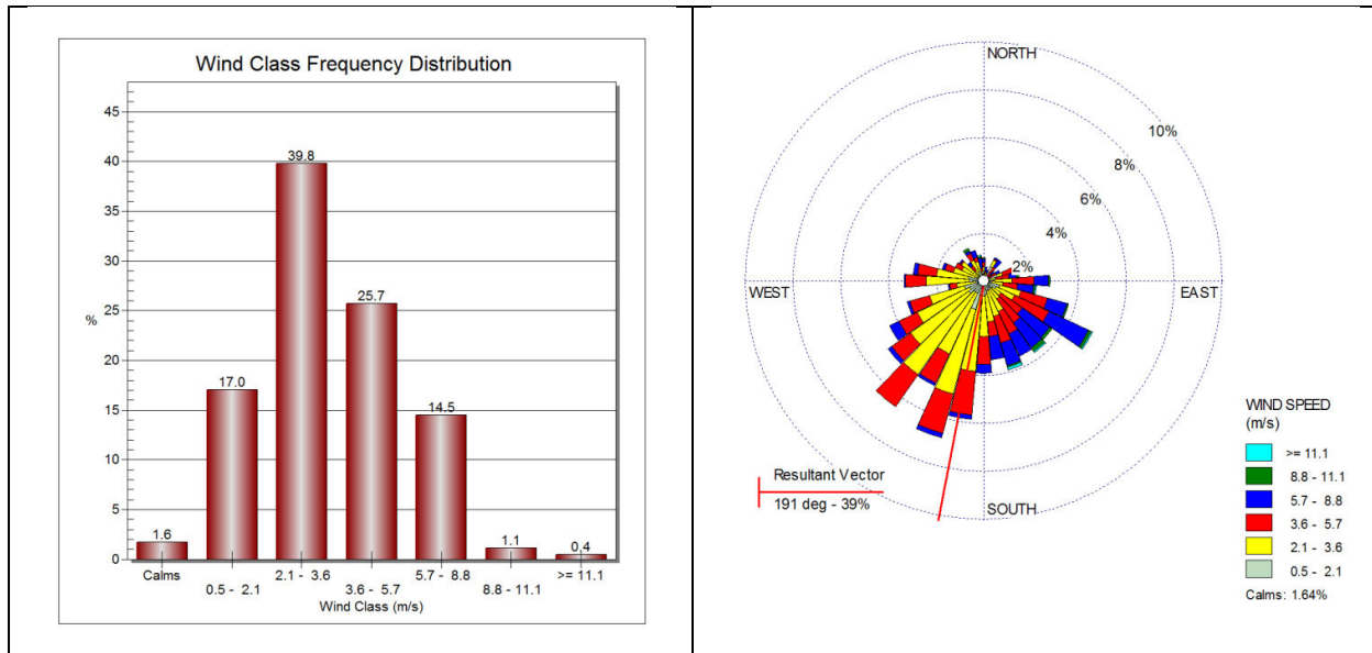
Figure No: 6.4 Wind Rose Diagram & Wind Class Distribution from 22 – 06 Hours
