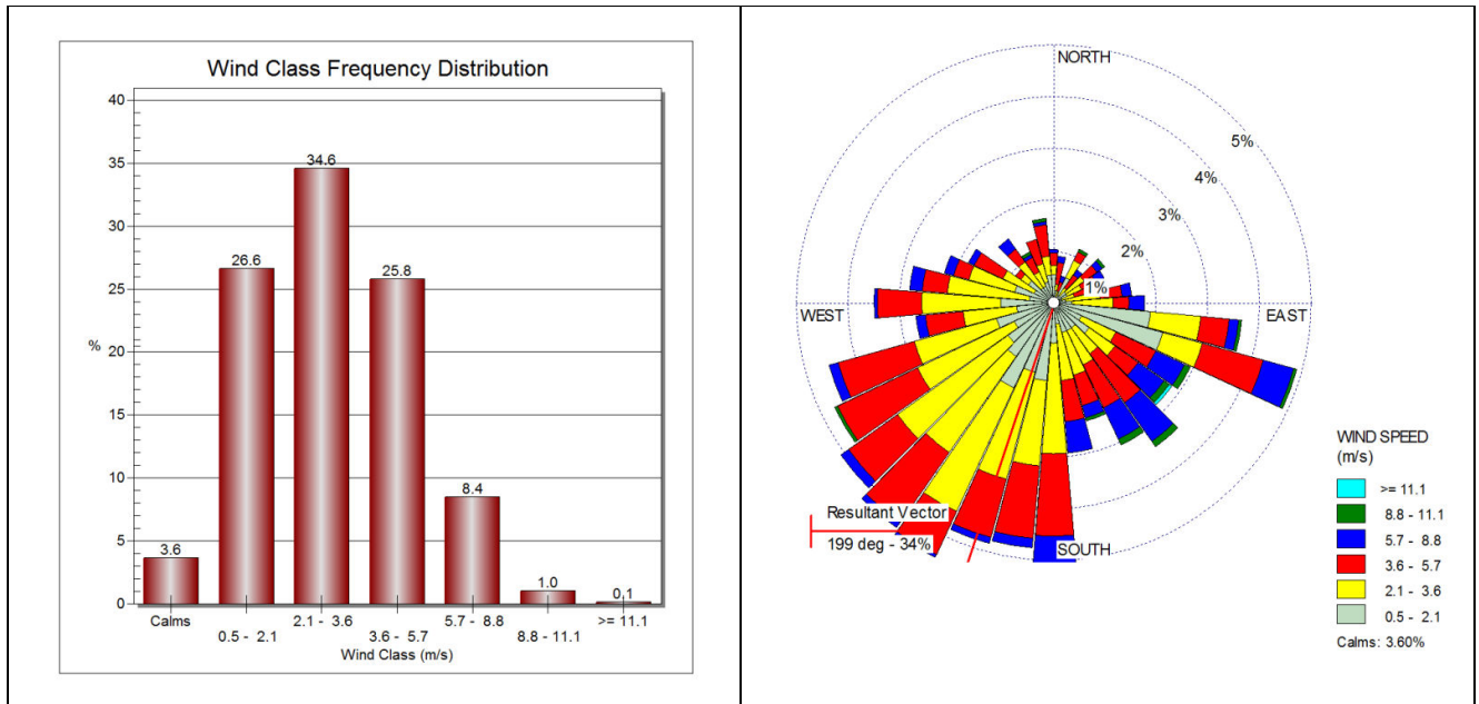
Figure No: 6.3 Wind Rose Diagram & Wind Class Distribution from 14 – 22 Hours
